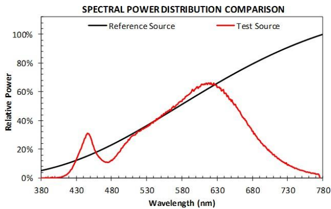
Spectral Power Distribution vs. Reference Source 3000K
