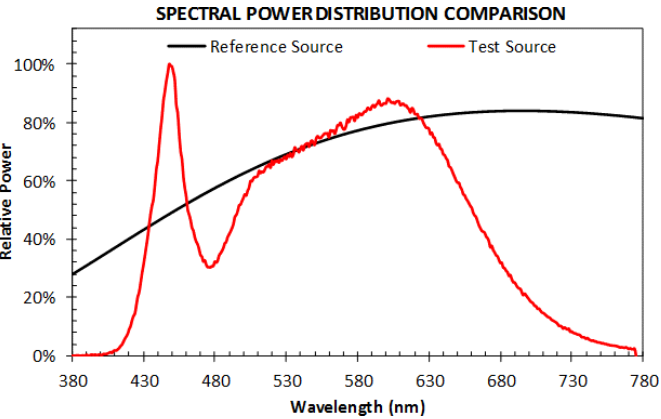
Spectral Power Distribution vs. Reference Source 4000K
